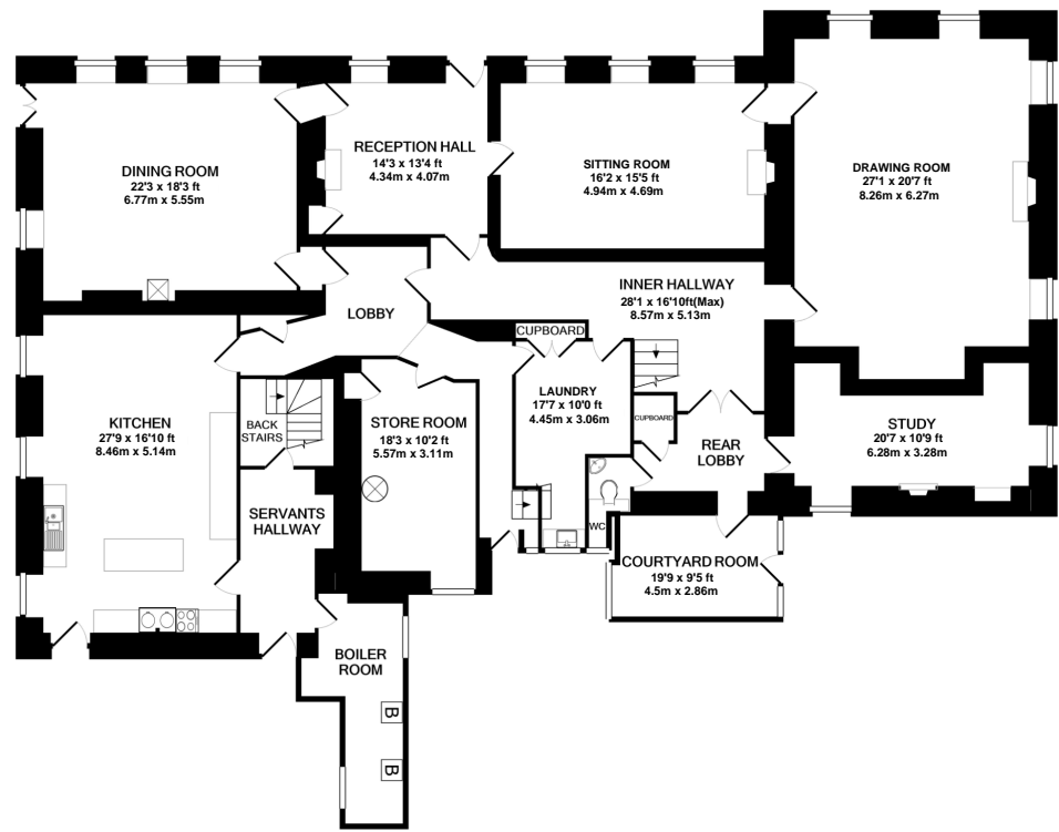
GROUND FLOOR AREA 3830.2sqft (355.84sqm)
