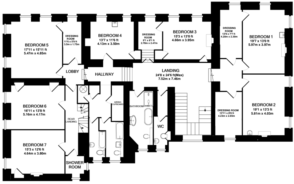
FIRST FLOOR AREA 3588.1sqft (333.35sqm)
