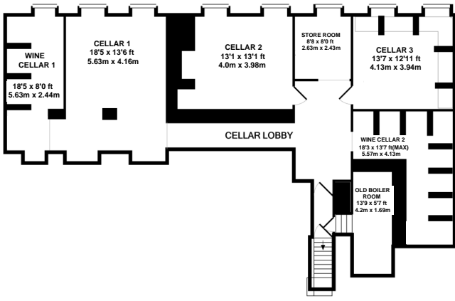
CELLAR AREA 1388.9sqft (129.03sqm)
