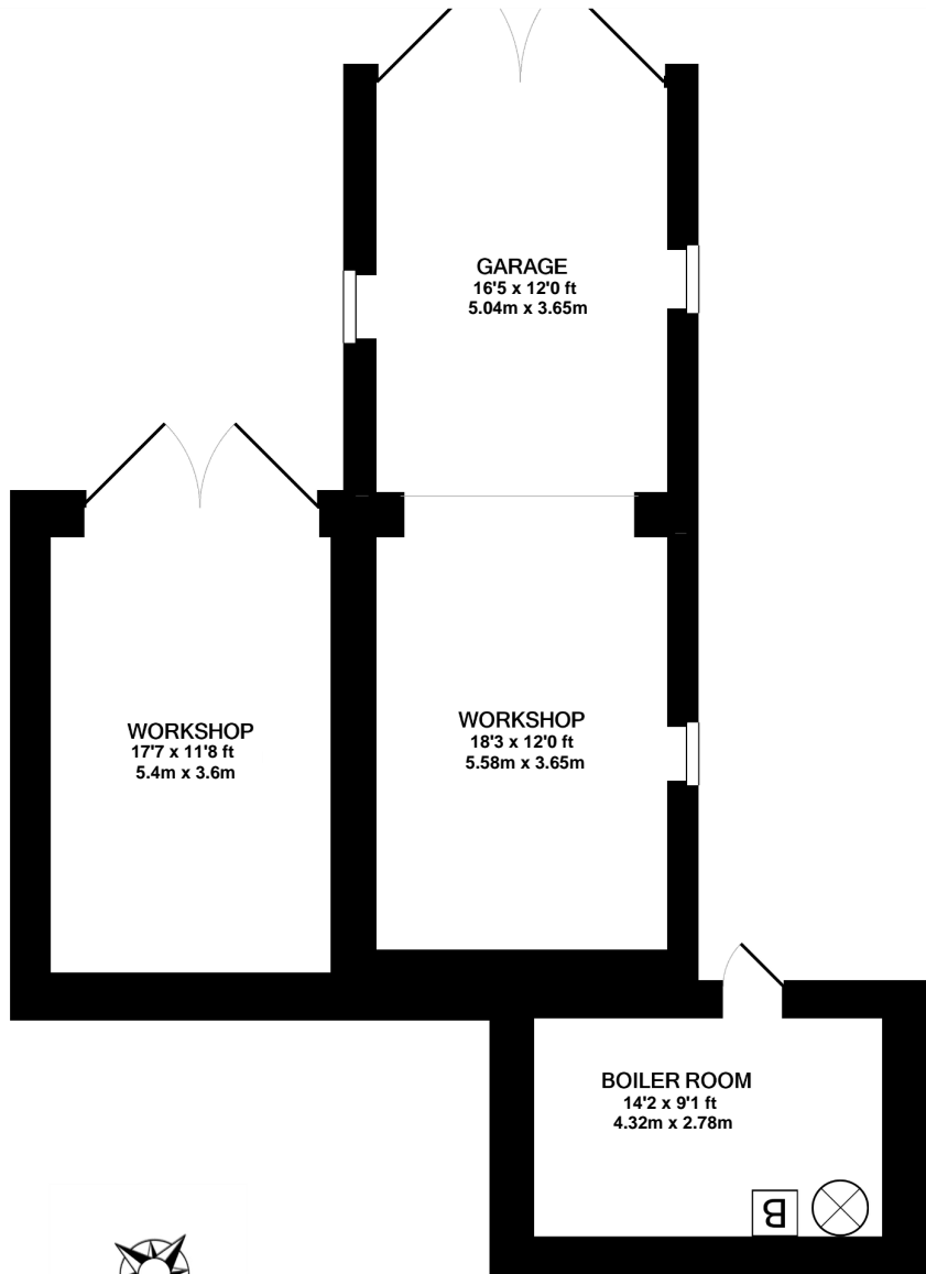
GROUND FLOOR AREA 757.9 sqft (70.41 sqm)
